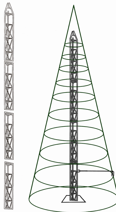
Trees 50 feet and over have an inner tower made of truss sections which provide more stability and accessibility for installation crews. Braces of several kinds may also be present.
